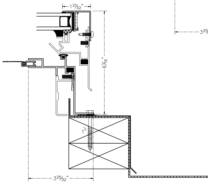
OPERABLE JAMB DETAIL
