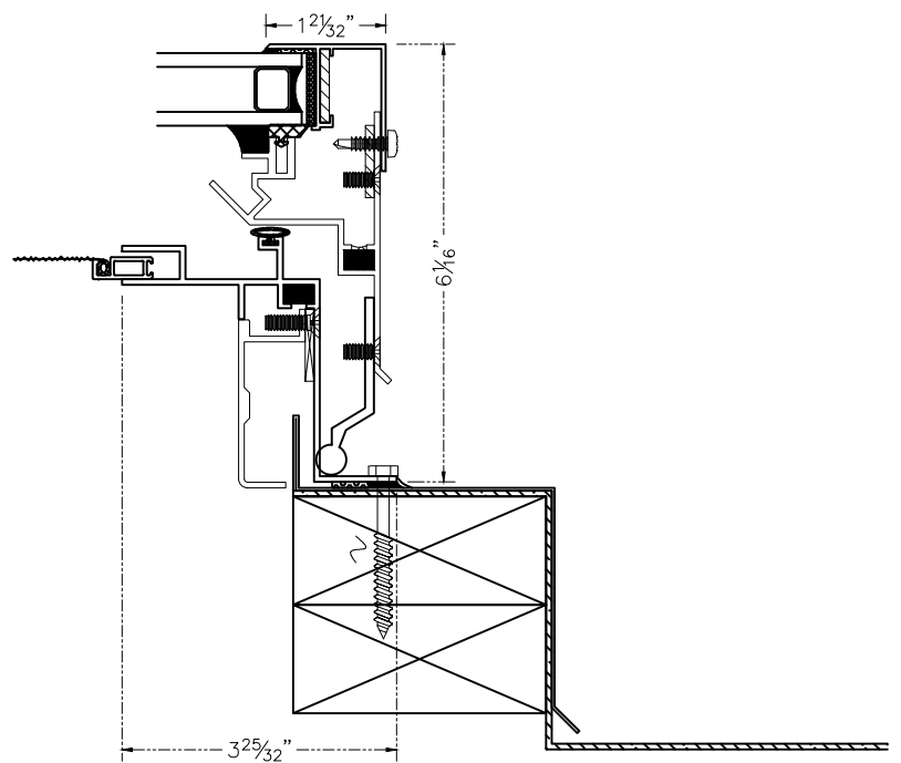
OPERABLE HEAD DETAIL
