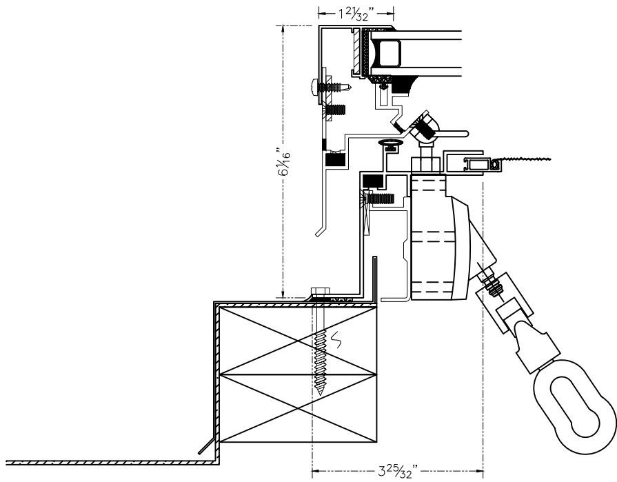
OPERABLE SILL DETAIL
