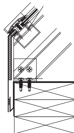
Pan Flashing Sill
