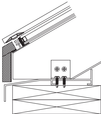
Extruded HD Curb Mount Sill
