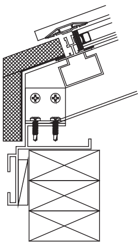
Standard Curb Mount Sill
