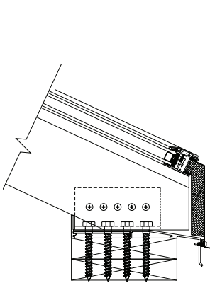
Extruded Curb
