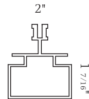
Boxed Muntin
