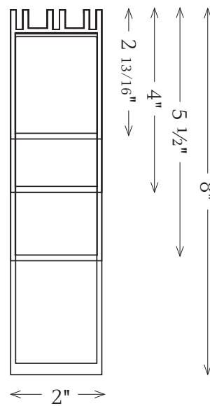
Boxed Muntin
