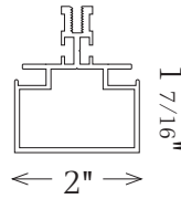
Boxed Muntin
