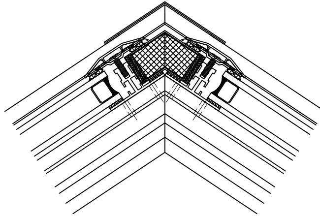
(X) RIDGE DETAIL 33.7° PITCH
