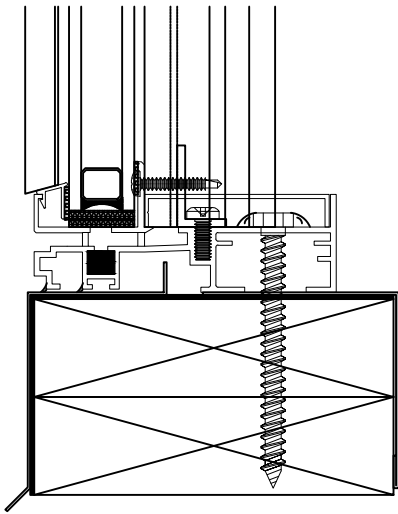
(X) REGULAR SILL RESTORATION
